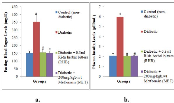
Fig 2: Effects of Rida herbal bitters on (a) fasting blood glucose levels (b) Insulin concentration in high-fat diet and STZ-induced diabetic rats. Values are expressed as mean ± SEM (n=8). *significant at p<0.05
